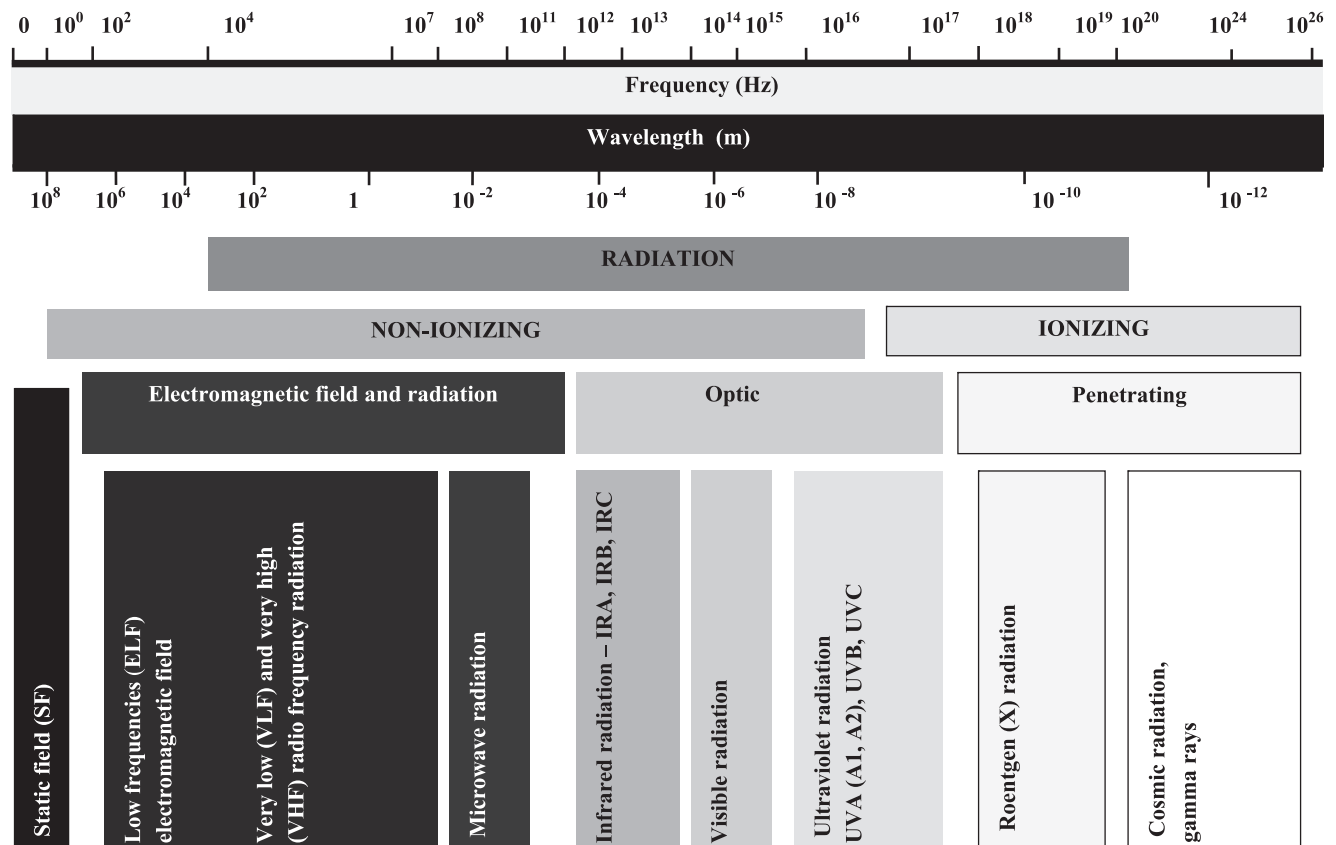
Fig. 1 – Electromagnetic spectrum. 13
