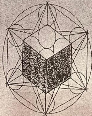
CUBE - EARTH
