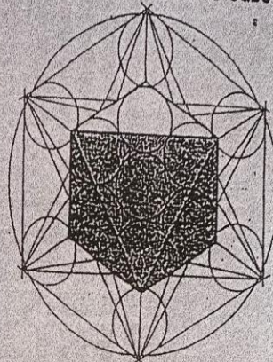
OCTAHEDRON - AIR
